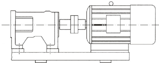
普通电机直接驱动 Directly driven by common motor
