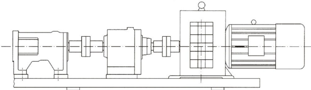
齿轮配合电磁调速电机驱动 Driven by gear with electromagnet adjustable motor
